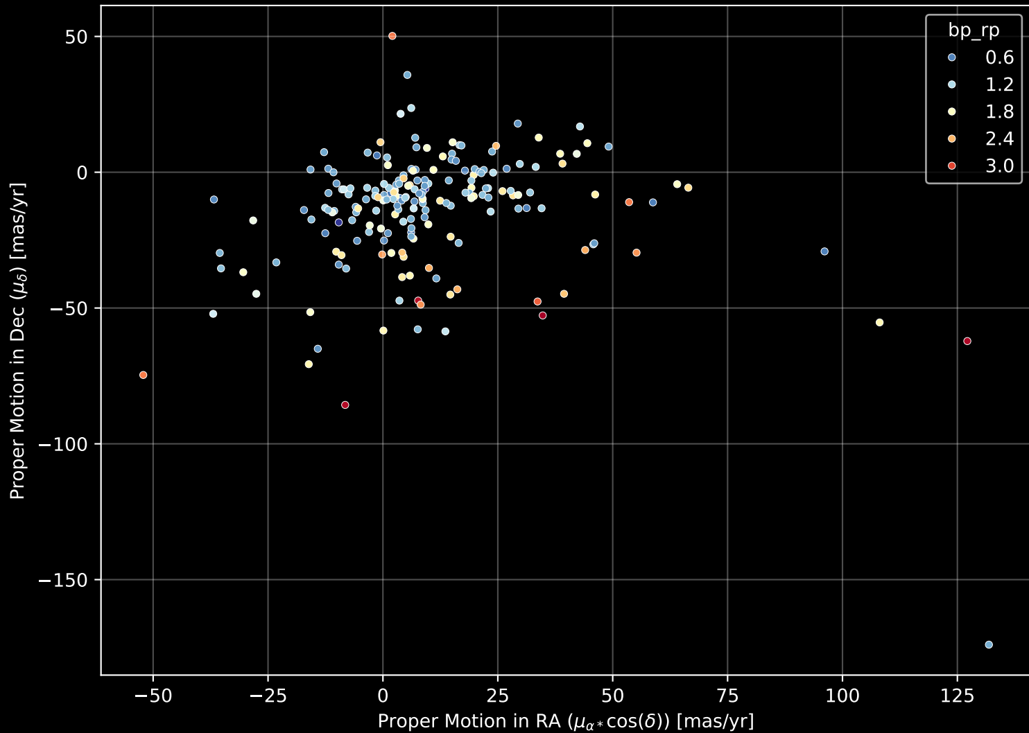
APOGEE DR17 Field: [K2_C3_053-50] Proper Motion Diagram (n= 200)
