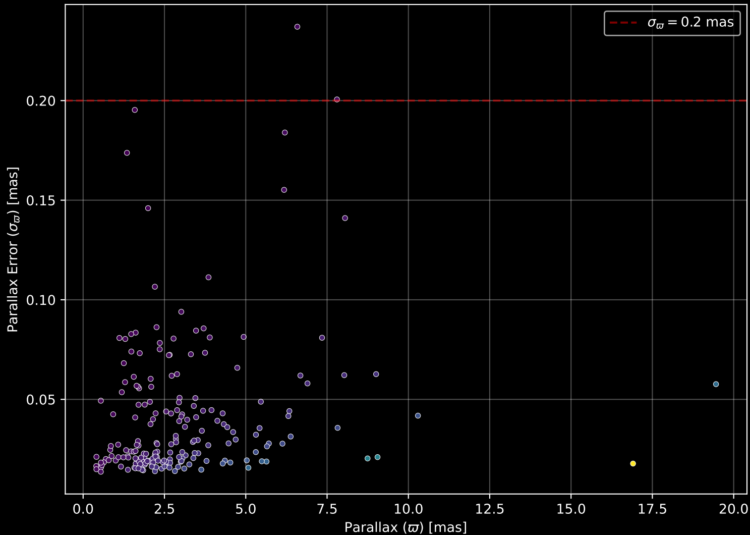
APOGEE DR17 Field: [K2_C3_053-50] Parallax Quality (n= 200)
