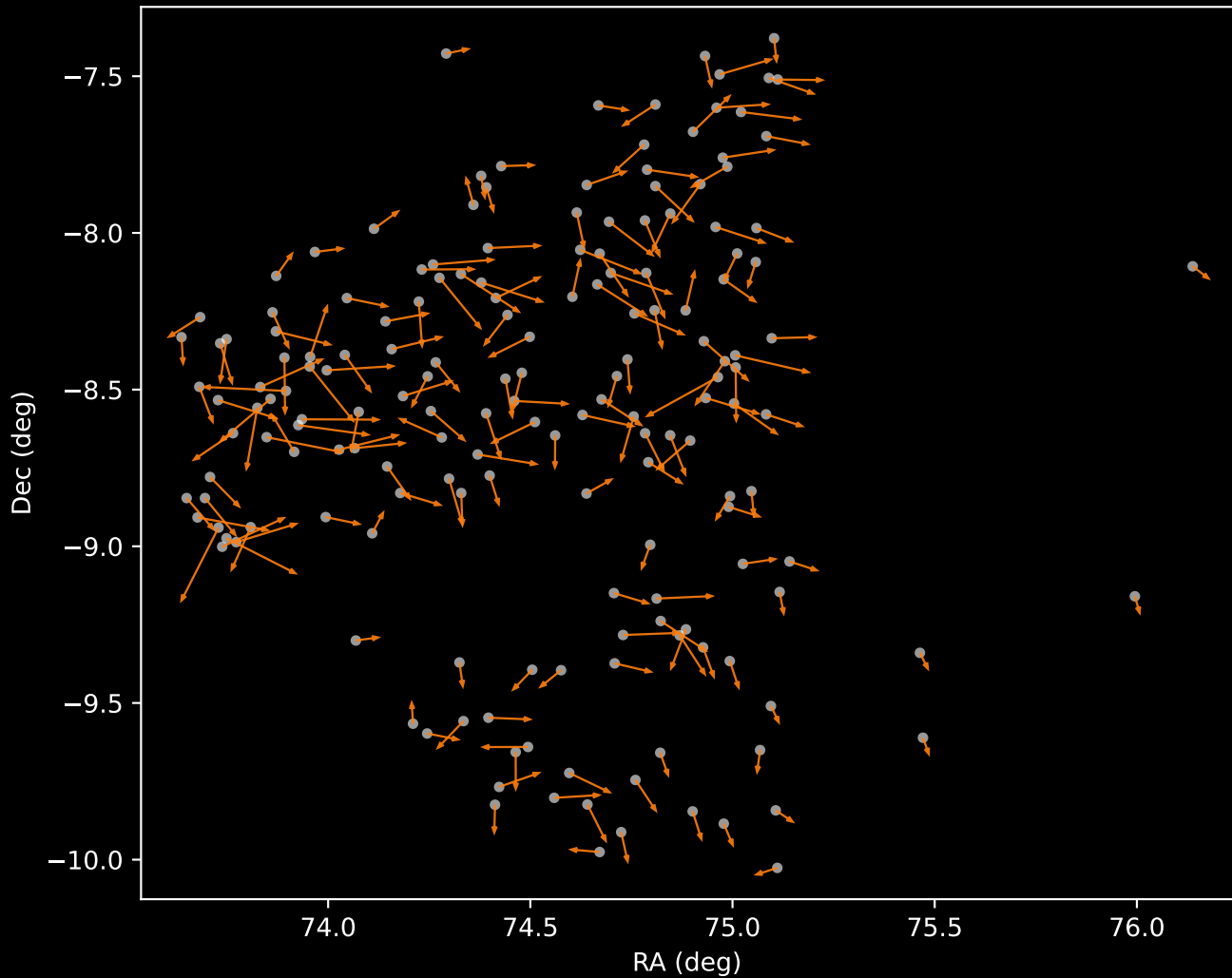
APOGEE DR17 Cluster 2 Proper Motion Vectors (n=174)
