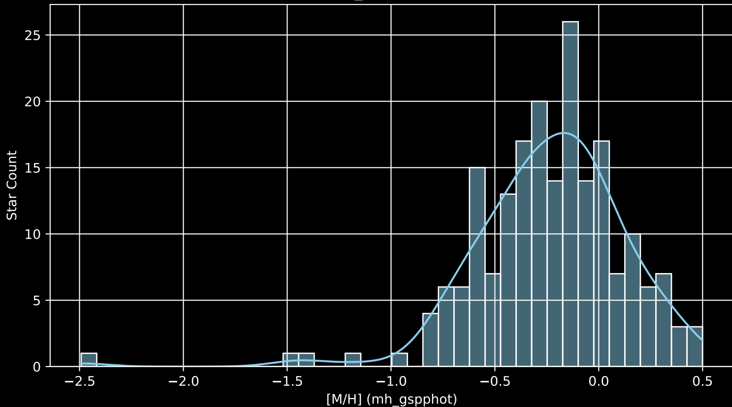
APOGEE DR17 Field: [K2_C3_053-50 [M/H] (mh_gspphot) (n= 200)
