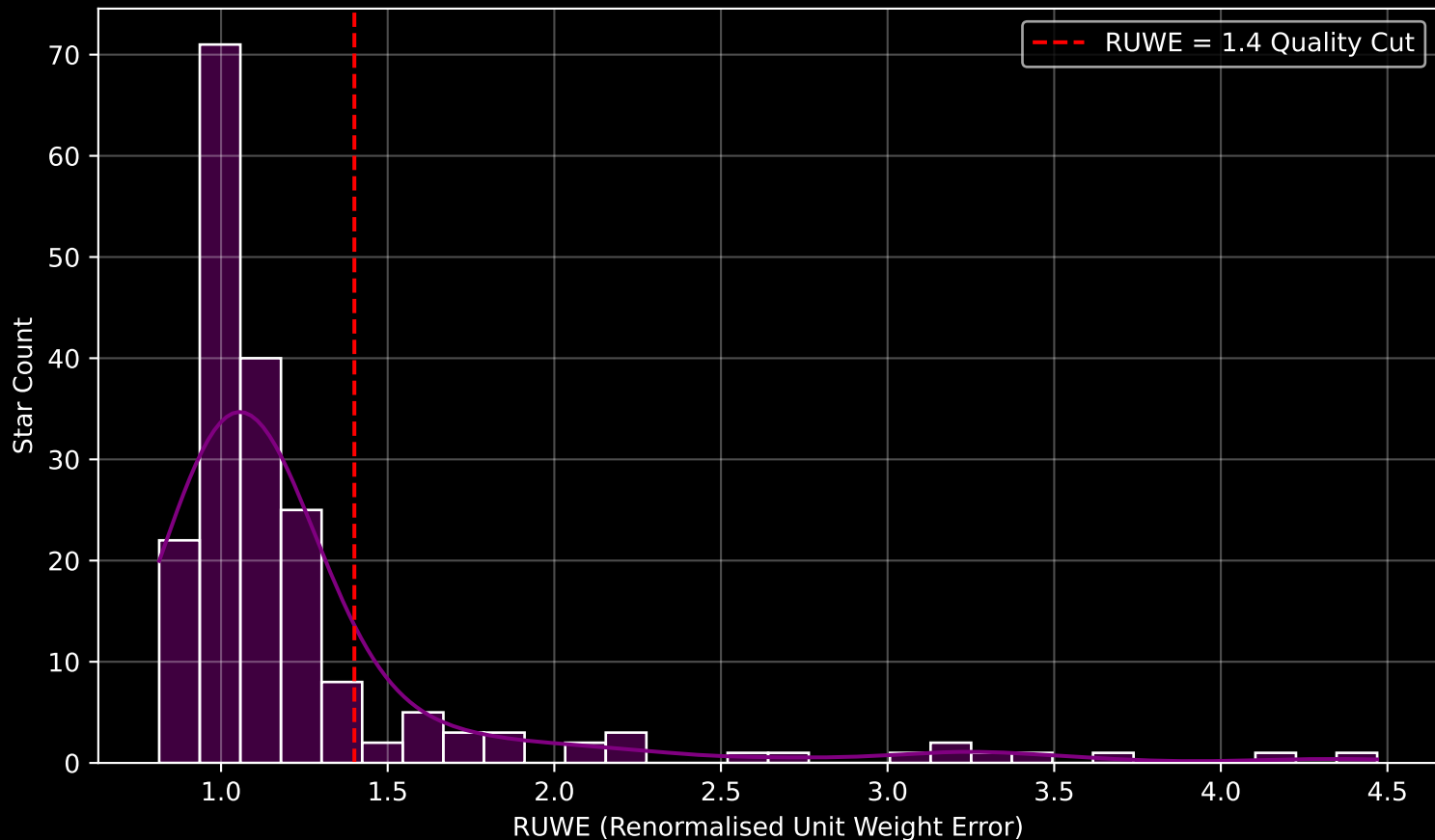
GAPOGEE DR17 Field [K2_C3_053-50] RUWE Distribution (n= 194)
