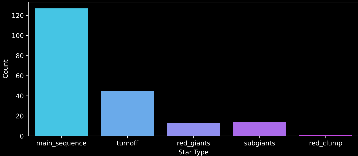
APOGEE DR17 Field: [K2_C3_053-50] Count plot of Star Type
