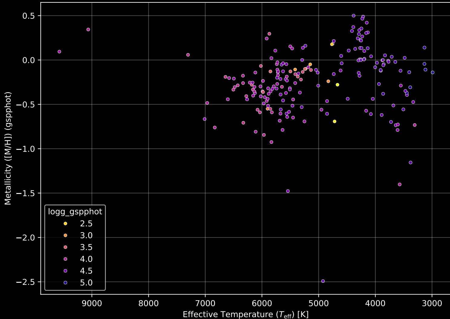
APOGEE DR17 Field: [K2_C3_053-50] Stellar Population Parameters (n= 200)
